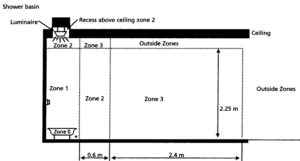
Elevation View
