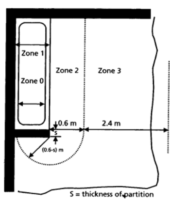
b) Bath tub, with permanently fixed partition
