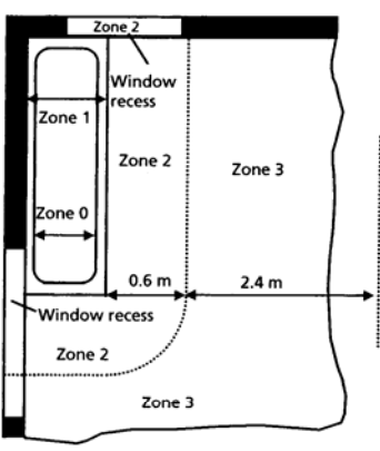
a) Bath tub
