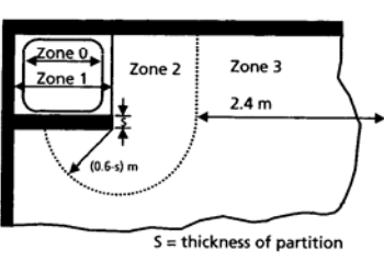
d) Shower basin with permanently fixed partition
